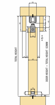
Installation Diagram
