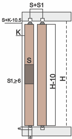
without rail end cup L=W
