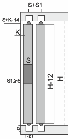
with rail end cup L=W-44
