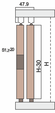
without rail end cup L=W
