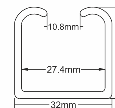
Sliding Track Diagram
